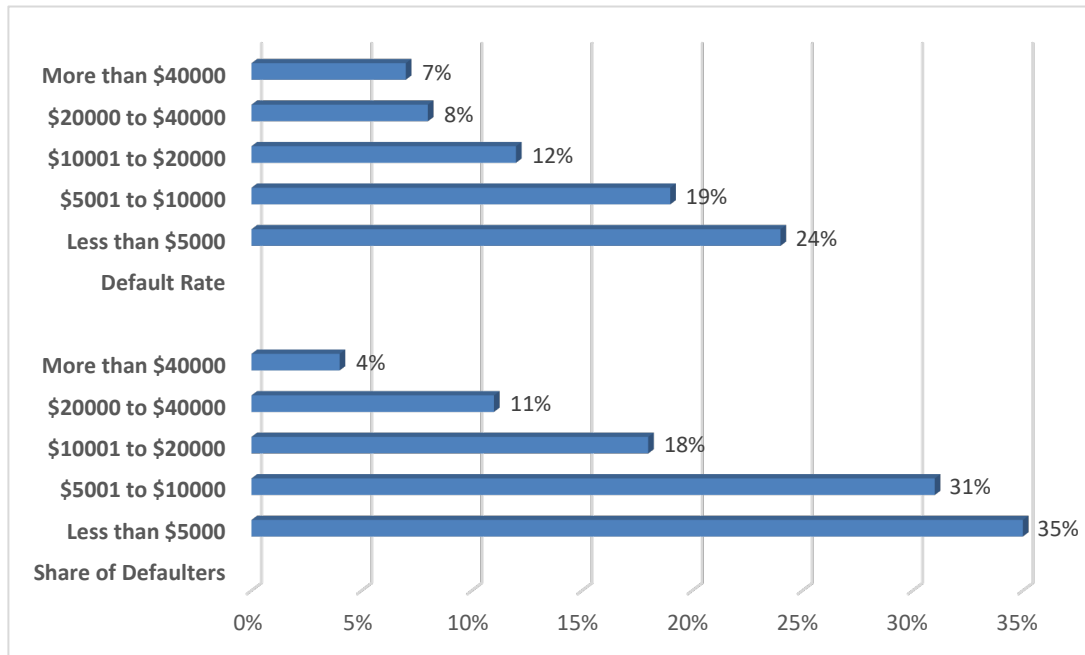
Figure 3: Share of Defaulters and Three-Year Federal Student Loan Default Rate Among Borrowers Entering Repayment in 2010–11, by Loan Balance
